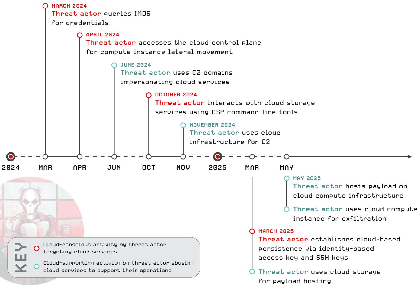
Figure 14. GENESIS PANDA: Weaponizing the cloud control plane
